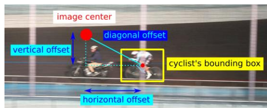
Figure 2. Evaluation process
