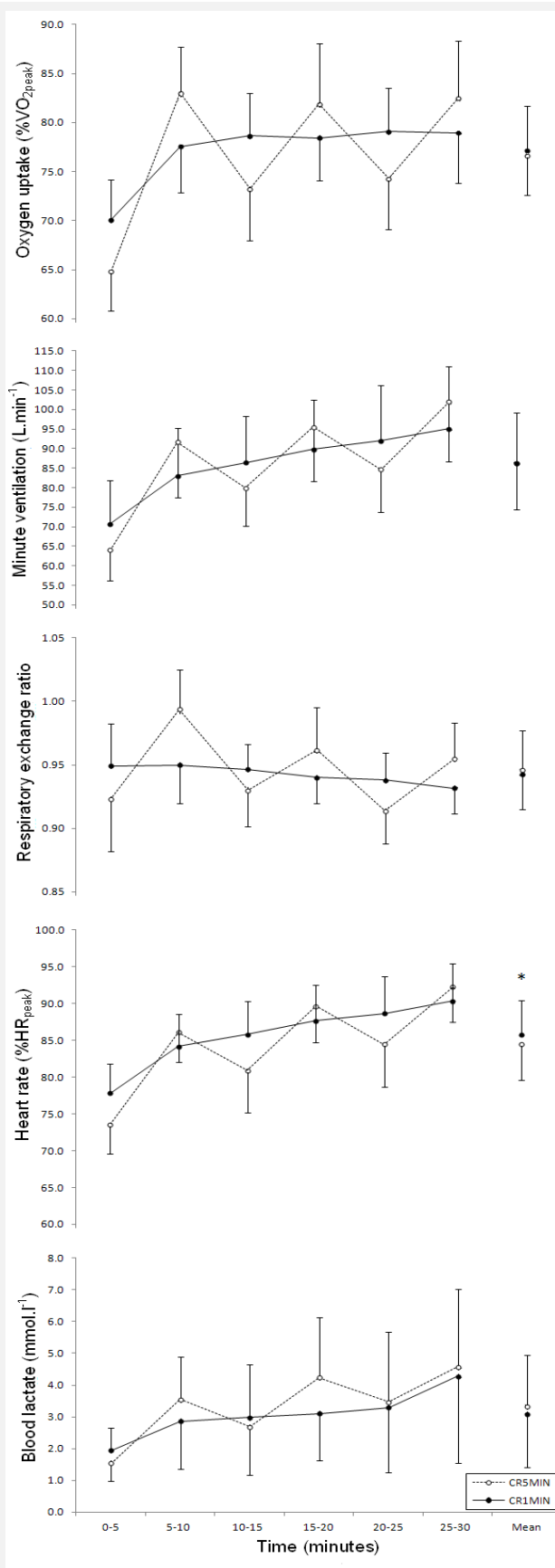
Figure 1 Epoch and mean values for cardiorespiratory variables (oxygen uptake, ventilation, respiratory exchange ratio, heart rate) and blood lactate for the CR5MIN and CR1MIN cycle protocols. Values are mean \pm SD.
