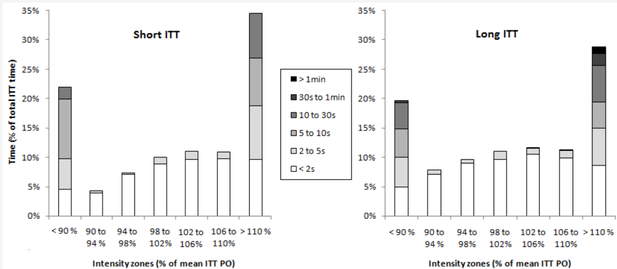
Figure 1: EVA analysis averaged for 3 professional cyclists on the same short and long Tour de France ITT
